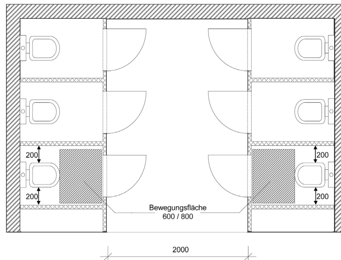
Double-row toilet facility, Outward-opening door (Dimensions in mm)
