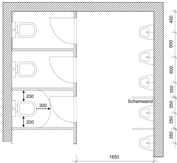
Single-row toilet facility with urinals, Inward-opening door (Dimensions in mm)
