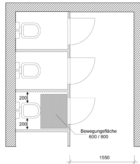
Single-row toilet facility, Door opening outwards (Dimensions in mm)
