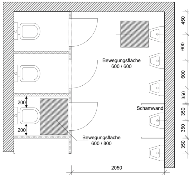
Single-row toilet facility with urinals, Outward-opening door (Dimensions in mm)
