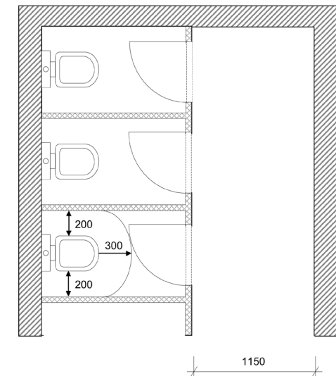
Single-row toilet facility, Door opening inwards (Dimensions in mm)
