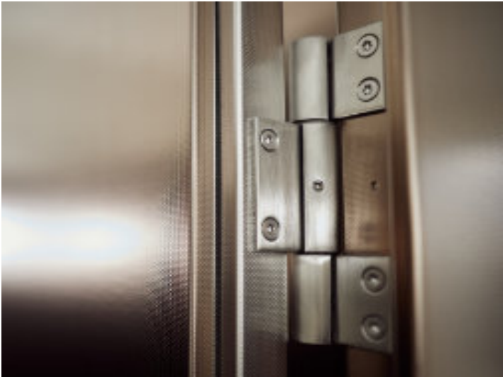
3-roller edge spring hinges made of stainless steel 304 (20 mm in diameter, length 145 mm)
