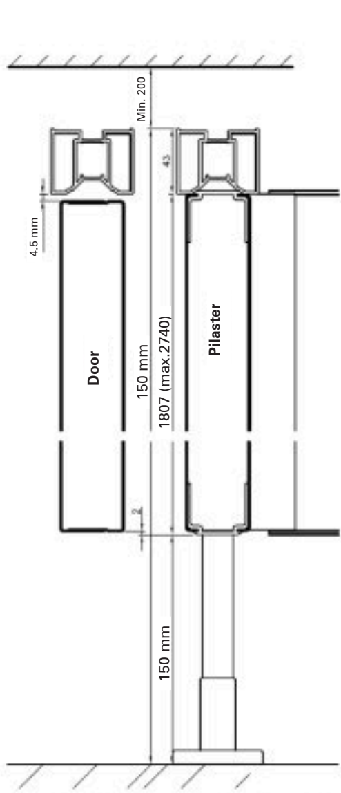
Section view of a standard configuration
