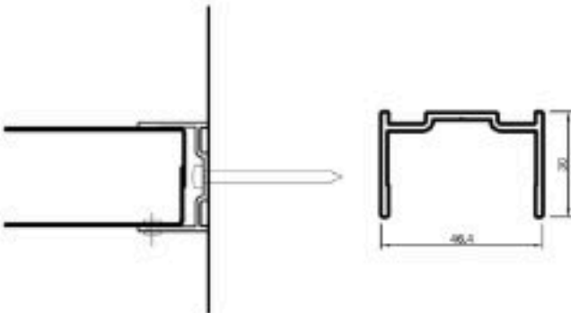
U-profile
