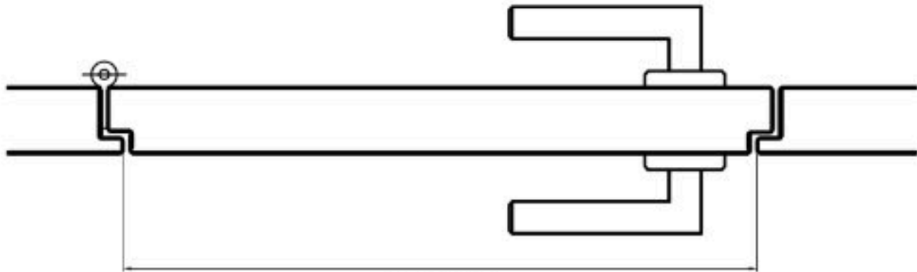
Nominal door width Mini 570 mm (22 7/16") / Maxi 980 mm (38 9/16") Door clear (in-swinging): - 52 mm (-2 1/16") Door clear (out-swinging): - 38 mm (-1 1/2")
