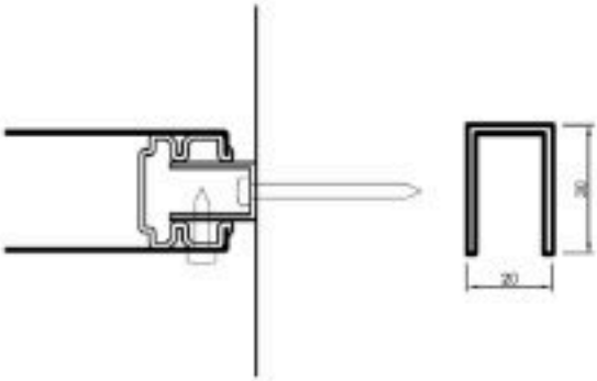
Shadow-gap profile (option)
