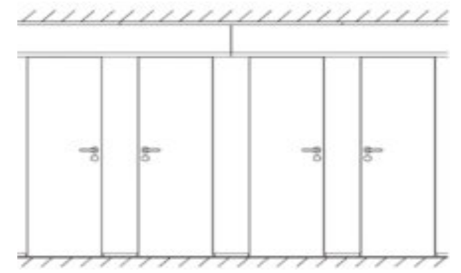
With continuous transom panel (possible height up to 3000 mm)
