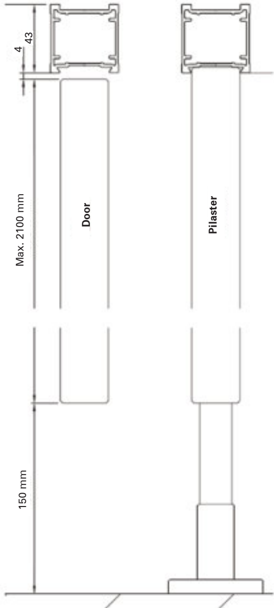
Section view of a standard configuration
