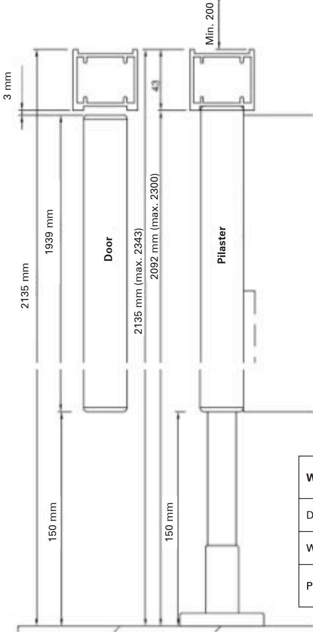
Section view of a standard configuration
